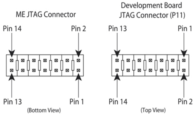
Bottom side of module (left) and development board from top (right)
