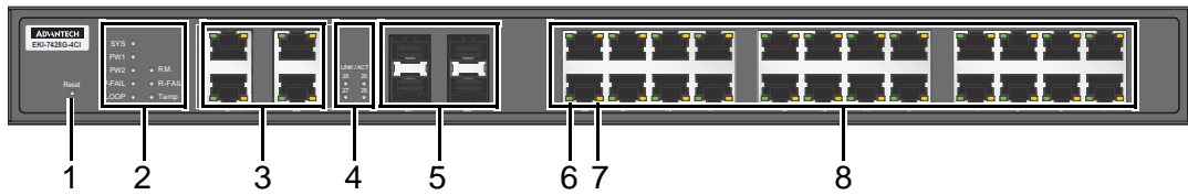
Figure 1.1 Front View
