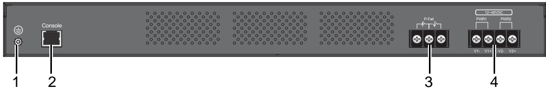
Figure 1.4 Rear View
