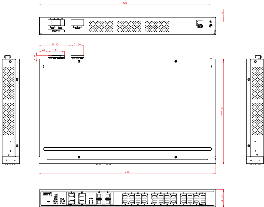
Figure 1.6 EKI-7428G-4CI Dimensions
