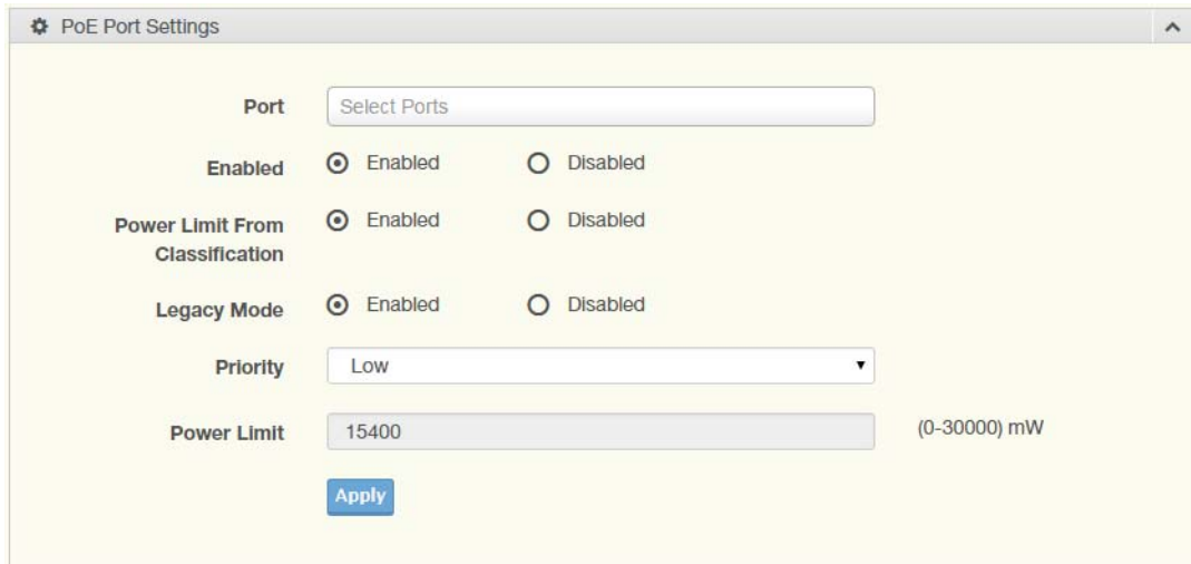
Figure 4.109 Management > Power Over Ethernet > PoE Port Settings
