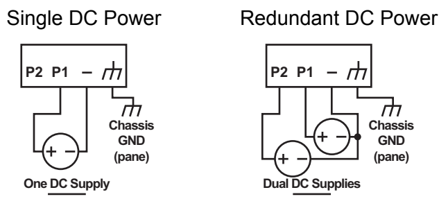
Figure 2.2 Power Wiring for EKI-9516 / 9512 Series
