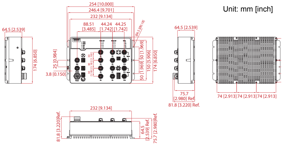
Figure 1.5 EKI-9512 Series Dimensions
