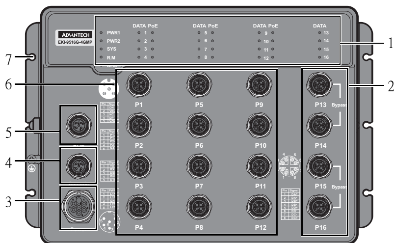
Figure 1.2 EKI-9516 Series Front View
