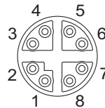
Figure 2.7 10/100/1000BaseT(X) Pin Assignment
