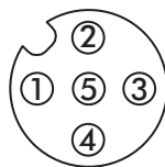
Figure 2.9 M12 A-Coded Connector Pin Assignment
