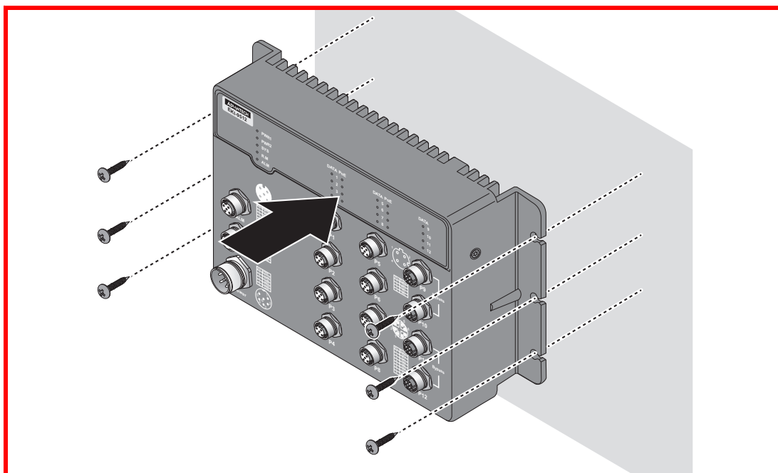
Figure 2.1 Switch Installation
