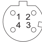
Figure 2.6 10/100BaseT(X) Pin Assignment
