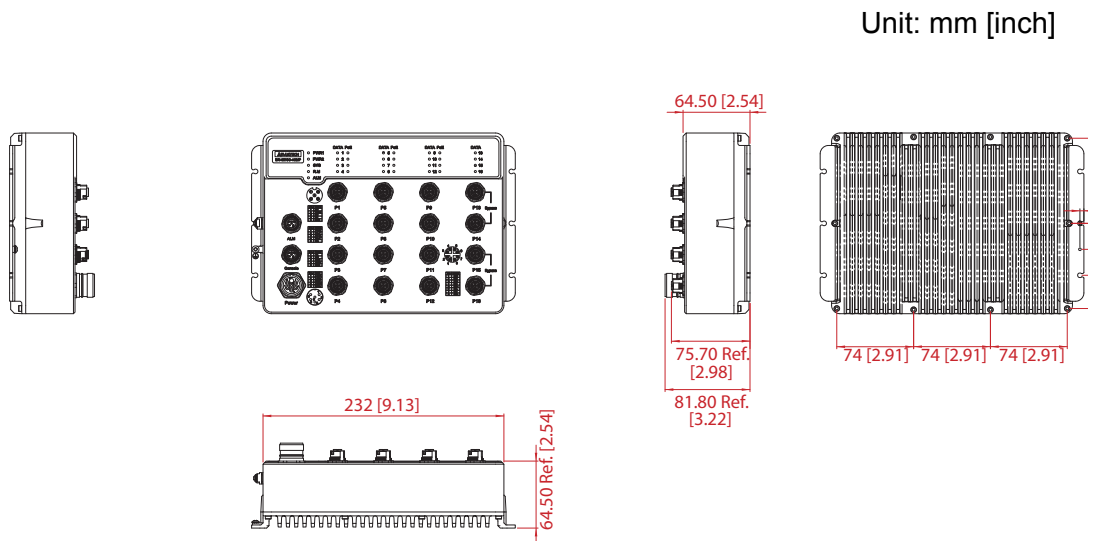
Figure 1.6 EKI-9516 Series Dimensions
