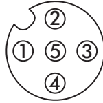
Figure 2.8 Alarm Contact Pin Assignment
