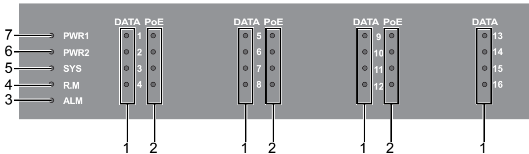
Figure 1.3 EKI-9512 Series System LED Panel
