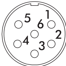
Figure 2.5 Standard M23 6-Pin Male DC Power Input Connector
