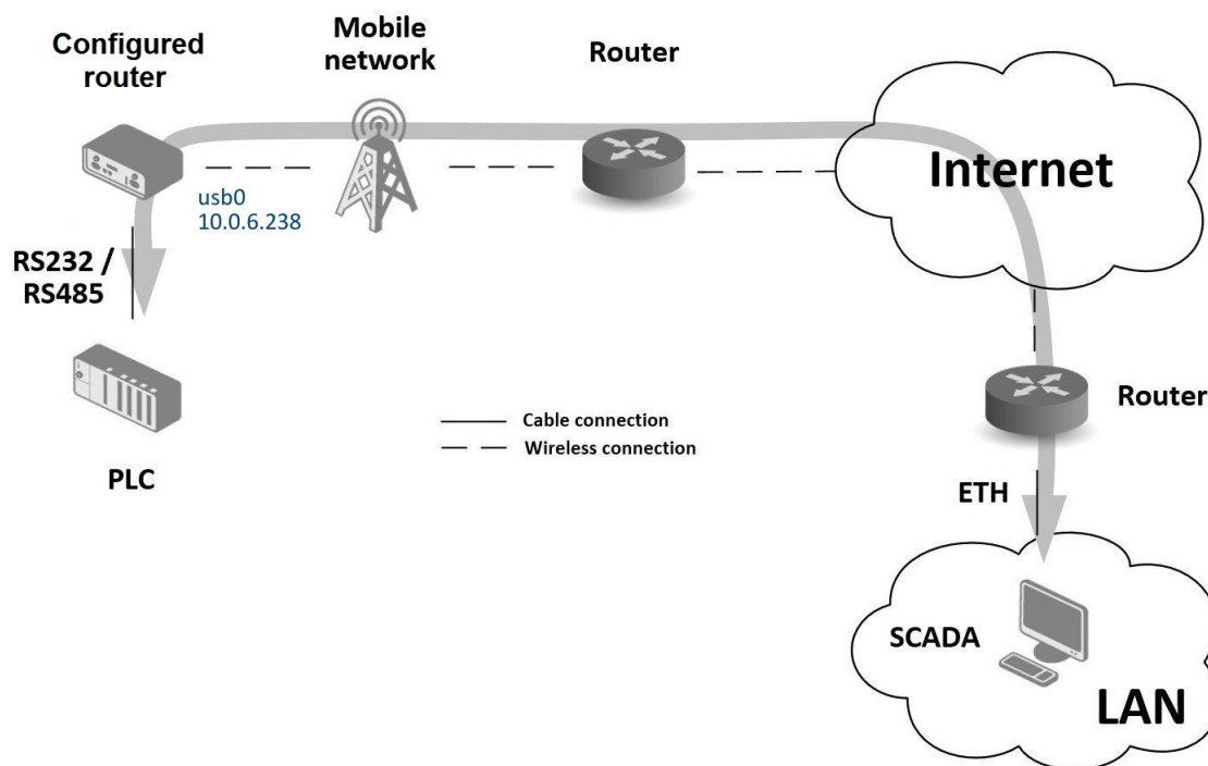
Figure 100: Serial Gateway – sample topology
