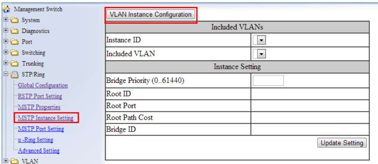
Figure 68: VLAN Instance Configuration
