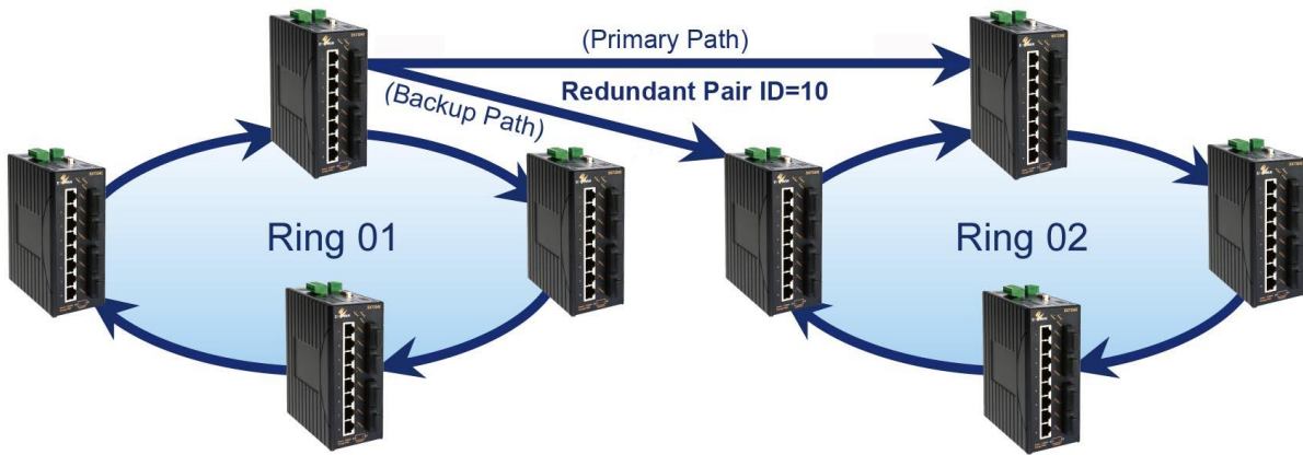
Figure 79: Redundant Pair Example 2
