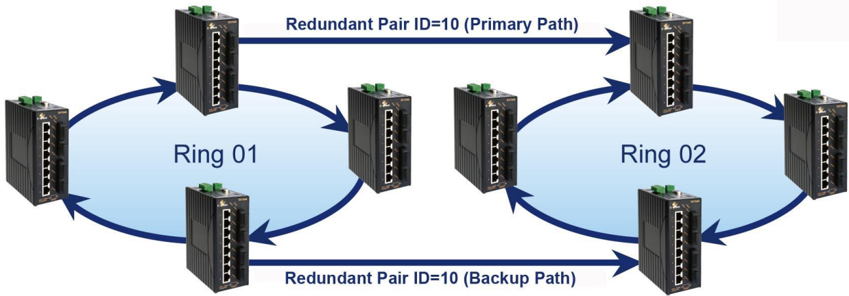
Figure 78: Redundant Pair Example 1
