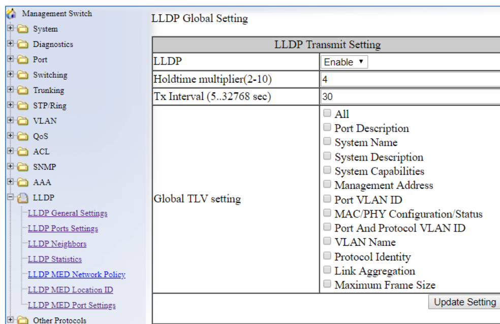
Figure 111: LLDP Global Settings
