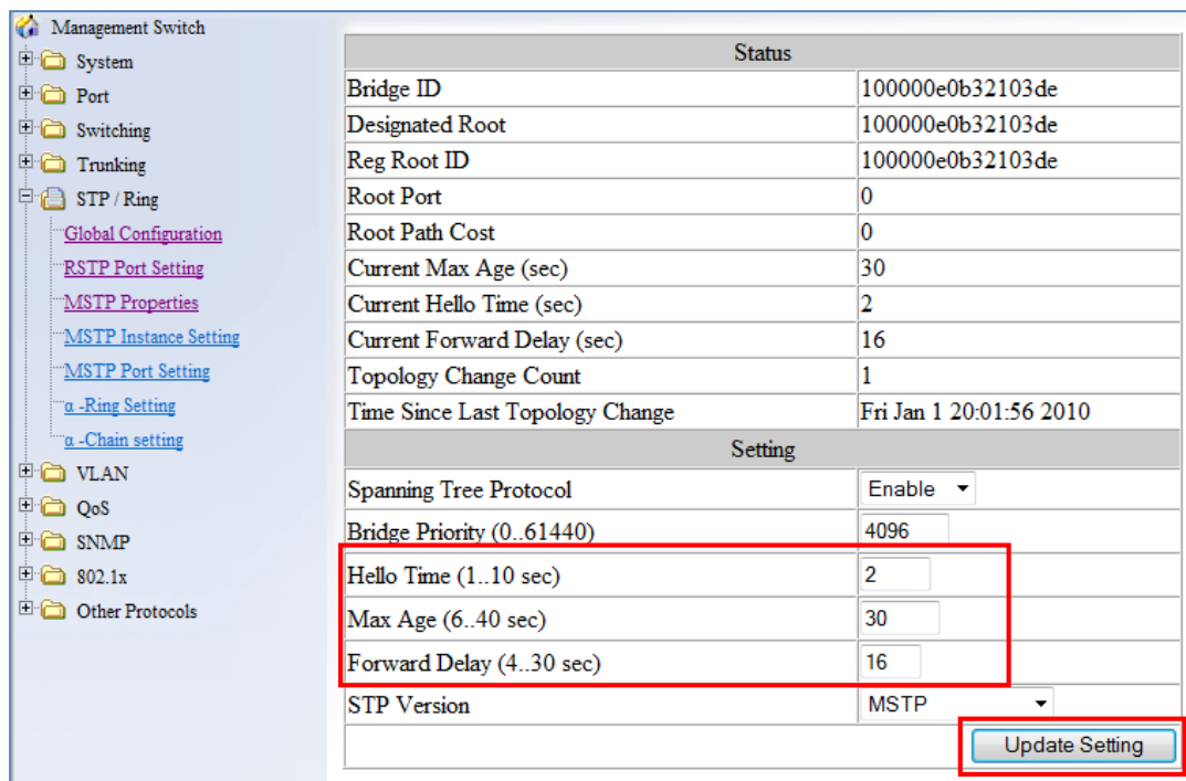
Figure 65: Max Age, Hello Timer & Forward Delay
