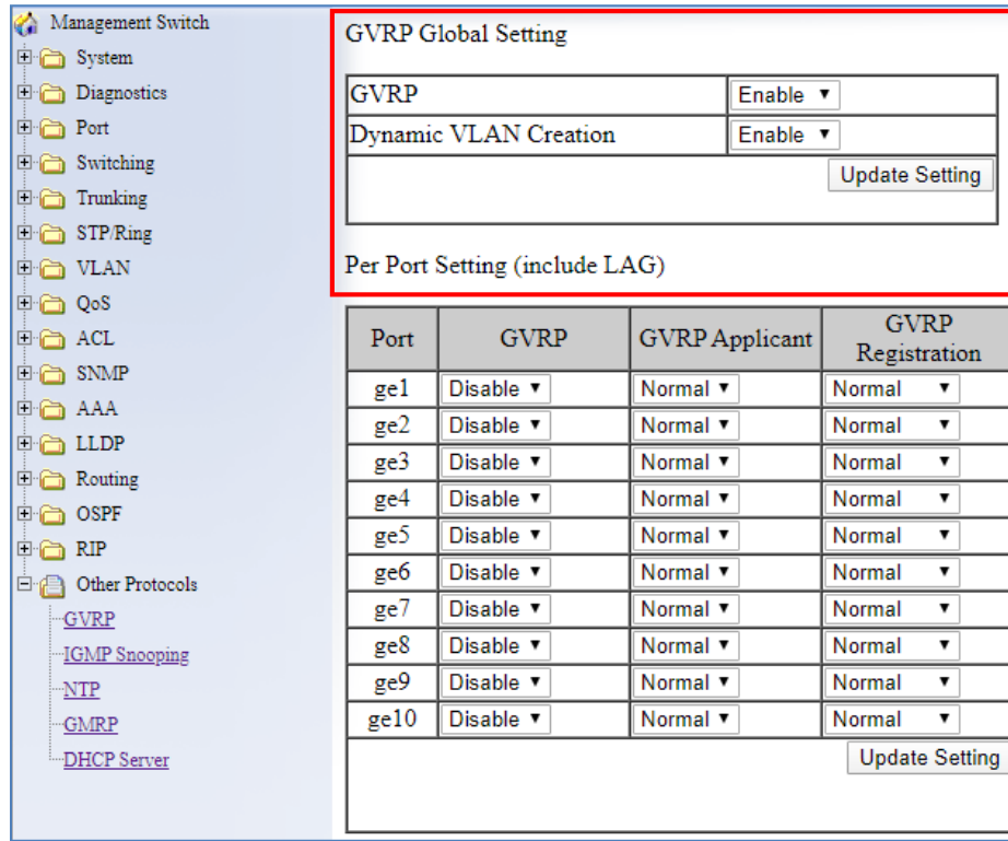
Figure 139: GVRP Configuration Distribution Switch
